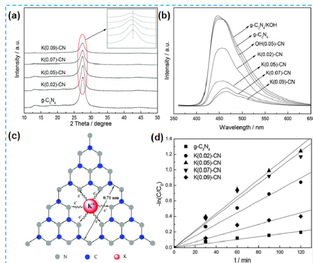
Fig. 2 (a) XRD patterns of the as-prepared CN and K(x)-CN. (b) PL spectra of the as-prepared CN-based catalysts. (c) Possible doping site for K ions in K(x)-CN. (d) The degradation of RhB under visible-light irradiation. 31
