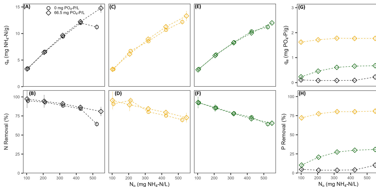
Fig. 2 Equilibrium NH 4 sorption after contact with Na-PT CZ (A), Ca-PT CZ (C), and Mg-PT CZ (E) and their respective NH 4 removals (B, D and F). Contact with Na-PT CZ is shown in black, Ca-PT CZ is in yellow, and Mg-PT CZ is in green. Data is shown for two scenarios: without presence of PO 4 in bulk liquid (circle) and with an initial background PO 4 of P_0 = 66.5 \pm 0.6 mg P L -1 (diamond). The associated equilibrium sorption (G) and percent removal (H) of PO 4 after contact with Na-PT CZ, Ca-PT CZ, and Mg-PT CZ is also shown.
