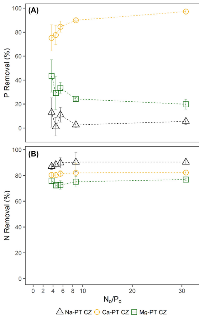
Fig. 3 \text{PO}_4 (A) and \text{NH}_4 (B) percent removal from tests 11–15 where the initial N/P ratios varied between 3.7–30.8.
