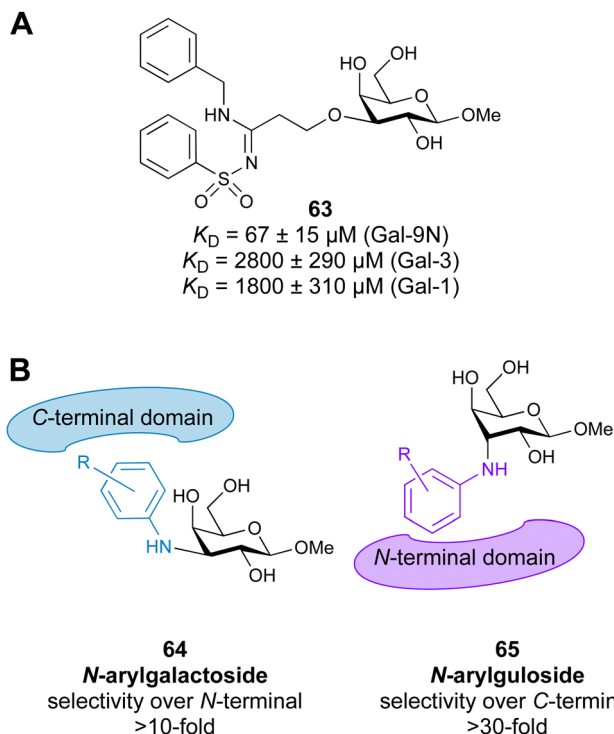
Fig. 12 Gal-9 inhibitors. (A) Galactoside- N -sulfonyl amidine, (B) selectivity switch between 3- N -aryl galactosides and 3- N -aryl gulcosides.
