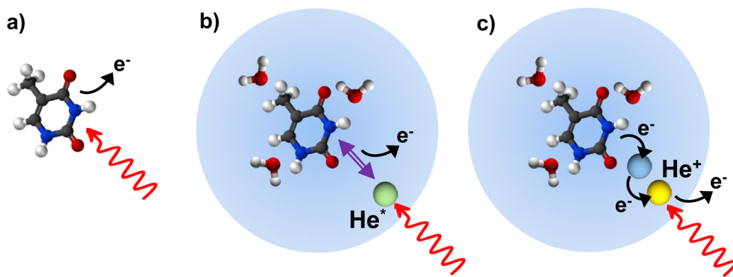
Fig. 2 Illustration of the three different ionization schemes for thymine and microhydrated thymine: (a) direct photoionization of the molecule, (b) Penning ionization in a helium nanodroplet following resonant excitation ( h\nu = 21.6 eV) of the droplet and (c) charge-transfer ionization in a helium nanodroplet after direct ionization of the droplet ( h\nu = 26 eV).
