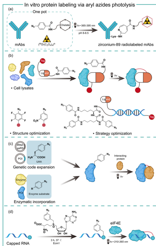
Fig. 5 In vitro protein labeling via aryl azides photolysis. (a) The aryl azides promoted photo-radiosynthesis of 89 Zr-radiolabelled monoclonal antibodies; (b) the aryl azides photoaffinity labeling of target proteins with structure and strategy optimization; (c) the incorporation strategies of aryl azides used in protein–protein photo-crosslinking; (d) the enzymatic incorporation of aryl azides in protein–RNA photo-crosslinking. mAbs, monoclonal antibodies; UAA, unnatural amino acid; aaRS, aminoacyl-tRNA synthetase; POI, protein of interest; Ecm1, encephalitozoon cuniculi mRNA cap (guanine N-7) methyltransferase; eIF4E, eukaryotic initiation factor 4E.
