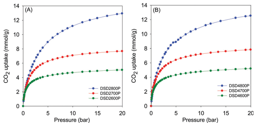
Fig. 5 CO 2 uptake isotherms of carbons directly compactated from sawdust (SD) at 600, 700 or 800 °C, and PO/SD ratio of 2 (A) or 4 (B).
