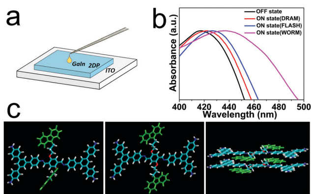
Fig. 5 (a) The schematic of the Ga-In/2DP/ITO device. (b) The UV-vis spectra of the device in different “ON” states and “OFF” state. (c) The proposed conformational change memory mechanism.
