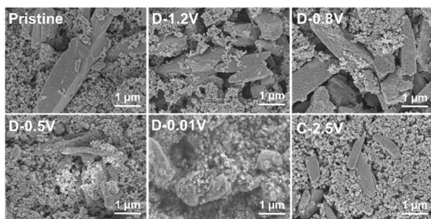
Fig. 6 SEM image of the Ni-DHBQ electrode recorded at different potentials.
