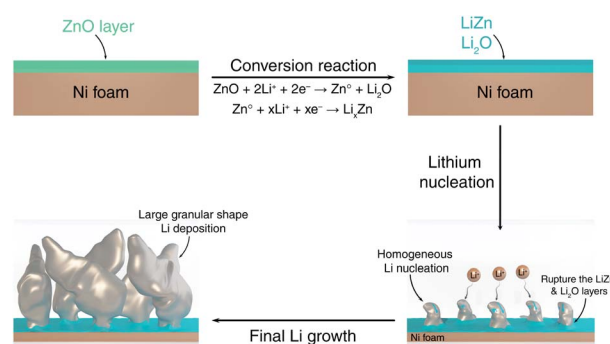
Fig. 6 Schematic illustration of the Li nucleation and growth on the ZnO-coated electrode.
