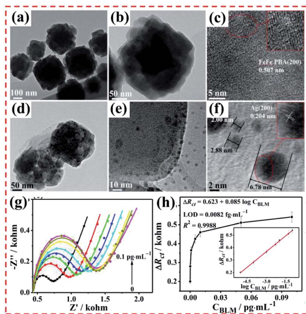
Fig. 26 TEM and HR-TEM images of (a–c) CuFe@FeFe and (d–f) AgNCs/Apt@CuFe@FeFe PBAs. (g) EIS responses of the AgNCs/Apt@CuFe@FeFe/Ag with different BLM concentrations. (h) Dependence of \Delta R_{ct} on the concentration of BLM based on AgNCs/Apt@CuFe@FeFe/Ag (inset: linear part of the calibration curve). Reproduced from ref. 192 with permission from the American Chemical Society, Copyright 2018.
