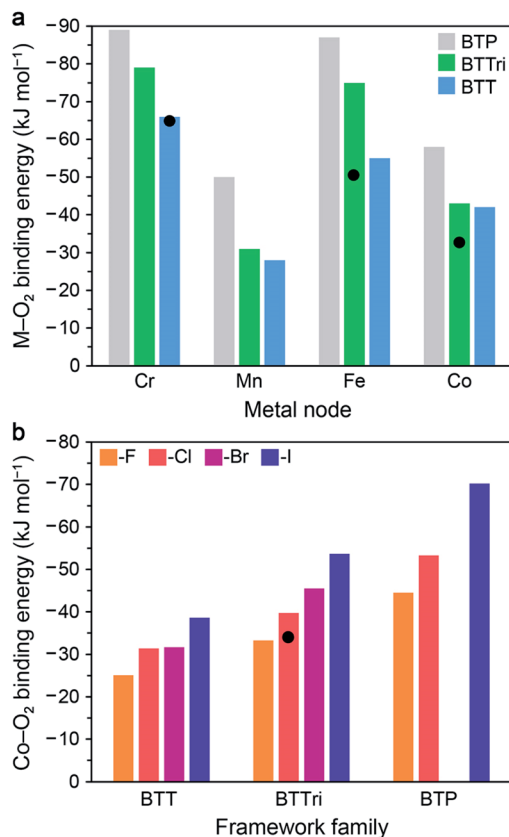
Fig. 5 (a) Results of DFT cluster calculations for O 2 binding energies in a series of model four-metal clusters [M_4Cl(\text{azolate})_8]^- ( M = \text{Cr}^{\text{II}} , \text{Mn}^{\text{II}} , \text{Fe}^{\text{II}} , and \text{Co}^{\text{II}} ; azolate = pyrazolate, triazolate, or tetrazolate to represent \text{BTP}^{3-} , \text{BTTri}^{3-} , or \text{BTT}^{3-} linkers). The TPSSh functional was used for M = \text{Mn}^{\text{II}} , \text{Fe}^{\text{II}} , and \text{Co}^{\text{II}} , and M06 was used for \text{Cr}^{\text{II}} (see Section S7.2 of the ESI† for details). Experimental enthalpy values are shown as black circles for Cr-BTT, Fe-BTTri, and Co-BTTri. As can be seen, TPSSh tends to overestimate experimental binding energies. Binding energies trend with the basicity of the azolate across all metals. (b) DFT calculations with periodic boundary conditions (PBE-D3 + U , U = 3.3 eV) for O 2 binding energies for the series of [(\text{Co}_4\text{X})_3(\text{benzenetrisazolate})_8] ( X = \text{F}^- , \text{Cl}^- , \text{Br}^- , and \text{I}^- ; benzenetrisazolate = \text{BTT}^{3-} , \text{BTTri}^{3-} , and \text{BTP}^{3-} ). The experimental O 2 binding enthalpy for Co-BTTri is shown as a black circle. Notably, binding energies trend with the electropositivity of the halide.
