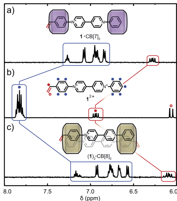
Fig. 2 Supramolecular complexation of 1^{2+} and CB[ n ]. 1 H NMR spectra of 1^{2+} at (a) \chi_{\text{CB}[7]} = 2 , (b) \chi_{\text{CB}[n]} = 0 and (c) \chi_{\text{CB}[8]} = 1 in \text{D}_2\text{O} . \text{Cl}^- counter-ions are omitted for clarity.
