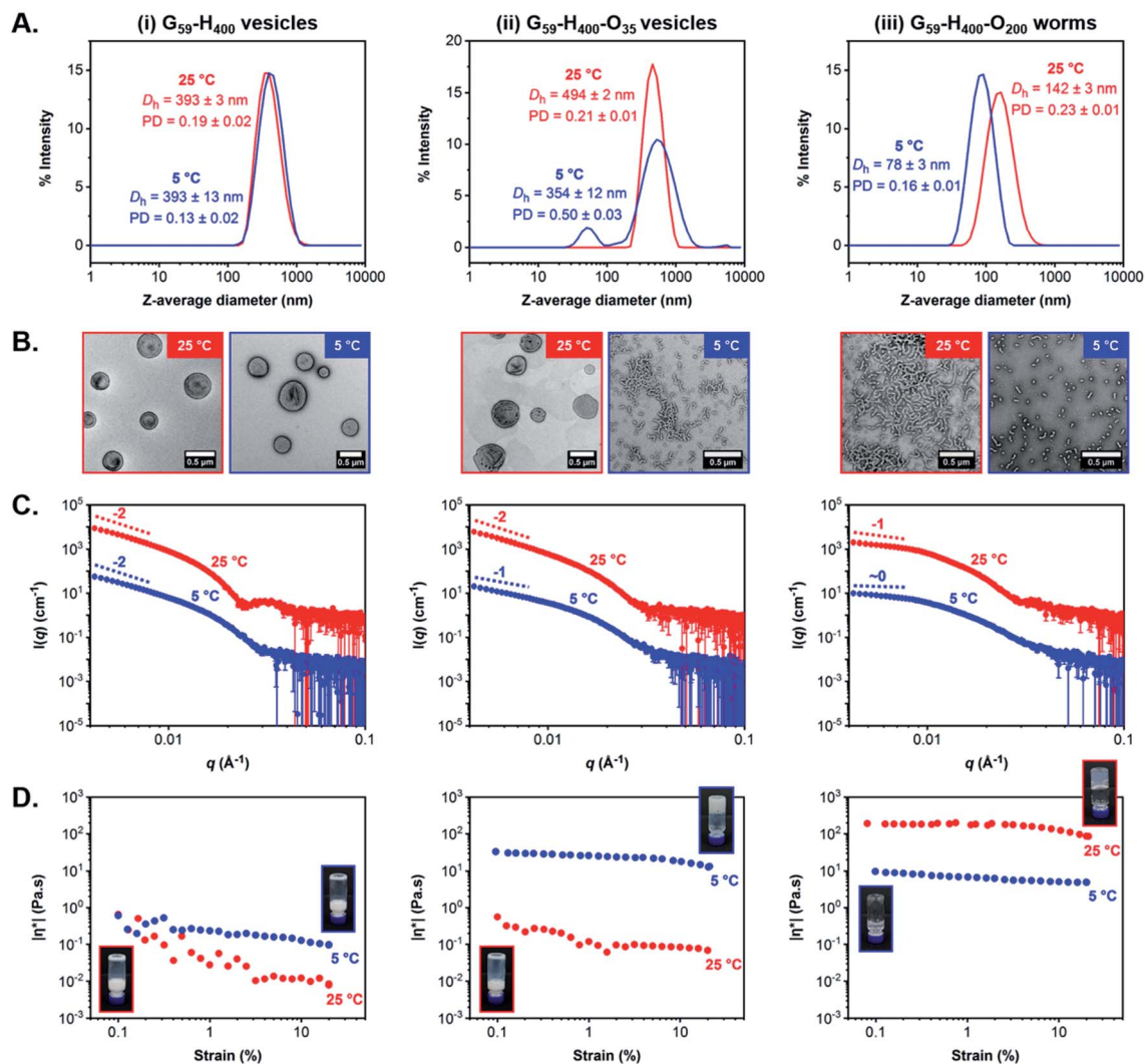
Fig. 5 Characterization data obtained for (i) G_{59}\text{-}H_{400} diblock copolymer vesicles, (ii) G_{59}\text{-}H_{400}\text{-}O_{35} triblock copolymer nano-objects, and (iii) G_{59}\text{-}H_{400}\text{-}O_{200} triblock copolymer nano-objects at 25 °C (red data) and 5 °C (blue data) after incubation at each temperature for 24 h prior to analysis: (A) intensity-weighted particle size distributions, mean D_h values and polydispersities determined by DLS analysis of 0.1% w/w aqueous dispersions (the error indicates the standard deviation from at least three repeat measurements). (B) Representative TEM images obtained using a uranyl formate stain. (C) SAXS patterns recorded for 1.0% w/w aqueous dispersions. (D) Complex viscosity ( |\eta^*| ) as a function of applied strain (insets show digital images recorded for the corresponding aqueous copolymer dispersions at 10–11% w/w solids, which indicate whether they form a free-standing gel or a free-flowing fluid in each case).
