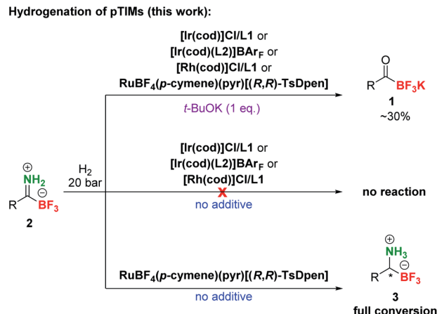
Scheme 3 Comparison of different reactivities of Bn-TiMs and pTiMs. Under the conditions that were successful in hydrogenation of the former, only partial hydrolysis to KAT was observed with model pTiM and an altogether different catalytic system was required. Catalyst and ligand structures are presented in Table 1.
