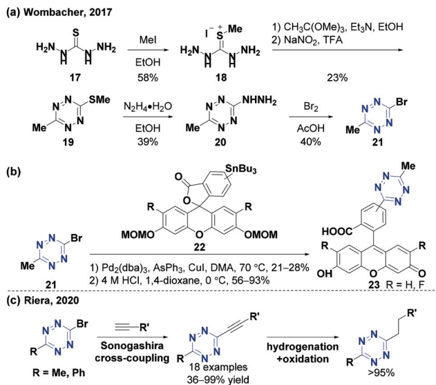
Fig. 3 Synthesis of tetrazine derivatives using 6-substituted bromotetrazines as starting building blocks. (a) Synthesis of 6-methyl bromotetrazine (21) from commercially available thiocarbohydrazide (17). (b) Synthesis of aryltetrazines from a bromotetrazine and a Sn-based reagent via Stille cross-coupling. (c) Sonogashira cross-coupling of bromotetrazines and terminal alkynes. OMOM: OMeOMe, TFA: trifluoroacetic acid, and DMA: N,N -dimethylacetamide.
