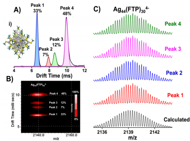
Fig. 7 (A) Drift time profile of \text{Ag}_{44}(\text{FTP})_{30}^{4-} ( m/z 2140) showing four peaks due to distinct isomeric structures with relative abundances of 33%, 7%, 12%, and 48%, respectively (calculated from peak area). Calculated structure of \text{Ag}_{44}(\text{SMe})_{30} is shown in inset (i). (B) Four well-defined spots observed in m/z vs. drift time plot. Each spot gave the same mass spectrum as shown in (C), matching with the calculated spectrum of the cluster. This figure has been reproduced from ref. 78 with permission from the American Chemical Society, copyright 2017.
