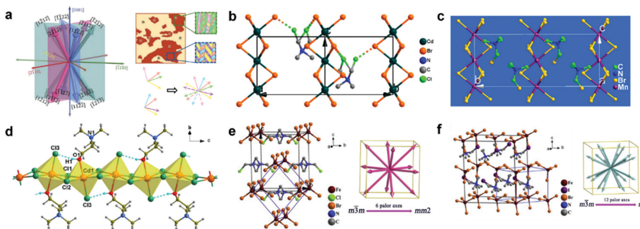
Fig. 5 Different structures of multiaxial ferroelectric halide perovskites. (a) Demonstration of twelve different polarization directions of the TMCM-MnCl 3 perovskite and the corresponding experimental evidence from PFM measurements. Reproduced with permission from ref. 48. Copyright 2017, American Association for the Advancement of Science. (b) Crystal structure of [(\text{CH}_3)_3\text{NCH}_2\text{Cl}]\text{CdBr}_3 in the ferroelectric phase. The dashed lines represent the Cl-Br interactions. Reproduced with permission from ref. 72. Copyright 2018, American Chemical Society. (c) Crystal structure of [(\text{CH}_3)_3\text{NCH}_2\text{X}]\text{MnBr}_3 in the ferroelectric phase. Reproduced with permission from ref. 73. Copyright 2017, American Chemical Society. (d) Crystal structure of [\text{Me}_3\text{NCH}_2\text{CH}_2\text{OH}]\text{CdCl}_3 with the edge-sharing \text{CdCl}_5\text{O} octahedra structure. The cations are coordinated alternatively above and below the perovskite framework. Reproduced with permission from ref. 74. Copyright 2020, American Chemical Society. (e) Crystal structure of (\text{TMCM})\text{FeBr}_4 and the corresponding six equivalent polarization directions. (f) Crystal structure of (\text{TMIM})\text{FeBr}_4 and the corresponding twelve equivalent polarization directions. Reproduced with permission from ref. 75. Copyright 2020, Elsevier.
