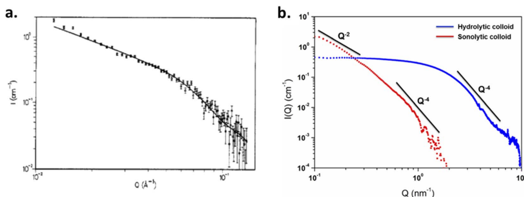
Fig. 10 (a) SANS diagram acquired on Pu colloids prepared in aqueous solution (total Pu 0.12 M) which measured 4.7 nm \times 190 nm according to data simulations. Adapted from ref. 100 with permission from the American Chemical Society, copyright 1990. (b) SAXS diagrams acquired for 10 mM hydrolytic and 0.8 mM sonolytic colloids. Black lines indicate the slope power laws. The slope observed for the hydrolytic colloid is typical for 3D objects and compact particles (2.6 nm according to simulations). The one observed for the sonolytic colloid is characteristic of elongated objects (e.g. thin disks or lamellas measuring 5.7 nm \times > 30 nm according to simulations). Reproduced from ref. 94 with permission from the Royal Society of Chemistry, copyright 2020.
