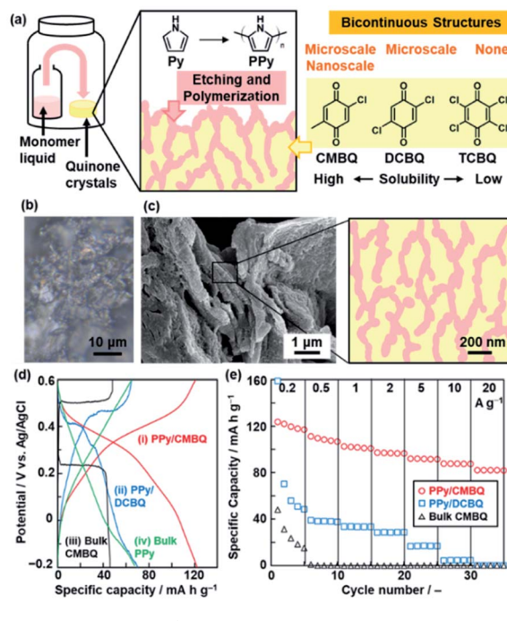
Fig. 5 Polymerization of the heteroaromatic monomer inside of the crystals. (a) Schematic illustration of the experimental setup, etching and polymerization on quinone crystals with diffusion of the monomer vapor, and morphological variation of the composites depending on the quinone derivatives with different solubilities in the monomer. (b) Cross-sectional optical-microscopy image of the pellet consisting of CMBQ crystals after the diffusion of the Py monomer. (c) SEM image and schematic illustration of the PPy/CMBQ microscale bicontinuous structure. (d) Charge–discharge curves of PPy/CMBQ (i, red line), PPy/DCBQ (ii, blue line), and the CMBQ bulk crystal (iii, black line) at 0.2 \text{A g}^{-1} . (e) Specific capacity of the PPy/CMBQ composite (red circles), PPy/DCBQ composite (blue squares), and commercial CMBQ bulk crystal (black triangles) at different current densities. Reproduced from ref. 23 with permission from the Royal Society of Chemistry.
