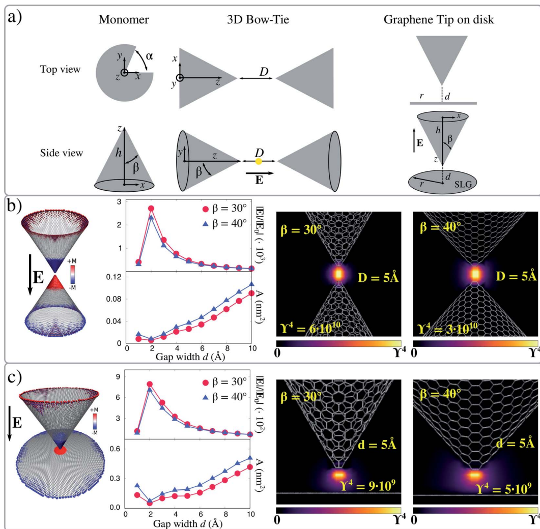
Fig. 3 (a) Geometrical parameters of graphene-based nanocones, 3D bow-ties and graphene tip-disks. (b) 3D bow-tie electric field enhancement factors ( |\mathbf{E}|/|\mathbf{E}_0| and \gamma^4 ) and localization area ( A ) for both \beta = 30^\circ and \beta = 40^\circ , as a function of the gap width ( D ) calculated at the boundary dipolar plasmon (see left panel) in the center of the gap. \beta = 30^\circ and \beta = 40^\circ electric field enhancement factors color map for 3D bow-tie nanostructure with D = 5 \text{ \AA} . (c) Graphene tip-disk electric field enhancement factors ( |\mathbf{E}|/|\mathbf{E}_0| and \gamma^4 ) and localization area ( A ) for both \beta = 30^\circ and \beta = 40^\circ , as a function of the gap width ( d ) calculated at the boundary dipolar plasmon (see left panel) in the center of the gap. \beta = 30^\circ and \beta = 40^\circ electric field enhancement factors color maps for graphene tip-disk nanostructure with d = 5 \text{ \AA} . The Fermi level is set to E_F = 0.4 \text{ eV} for each configuration.
