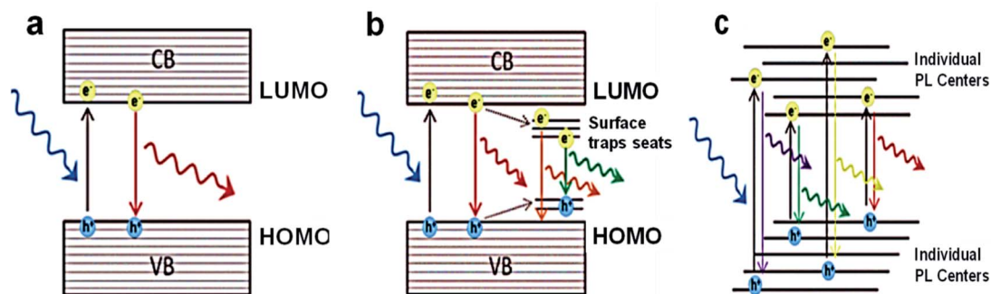
Fig. 4 Scheme of the various photoluminescence mechanisms and their unique characteristics: (a) SQUADS with quantum confinement, where the size-dependent PL, excitation-independent PL has narrow PL band and long lifetimes; (b) CDs/GQDs with quantum confinement, where the size-dependent and excitation-independent PL has a broad PL band and medium lifetimes; (c) CNDs with no quantum confinement, where the size-independent and excitation-dependent PL has a broad PL band and short lifetimes. 49 Adapted from ref. 49 with permission from the Royal Society of Chemistry (Great Britain), copyright 2021.
