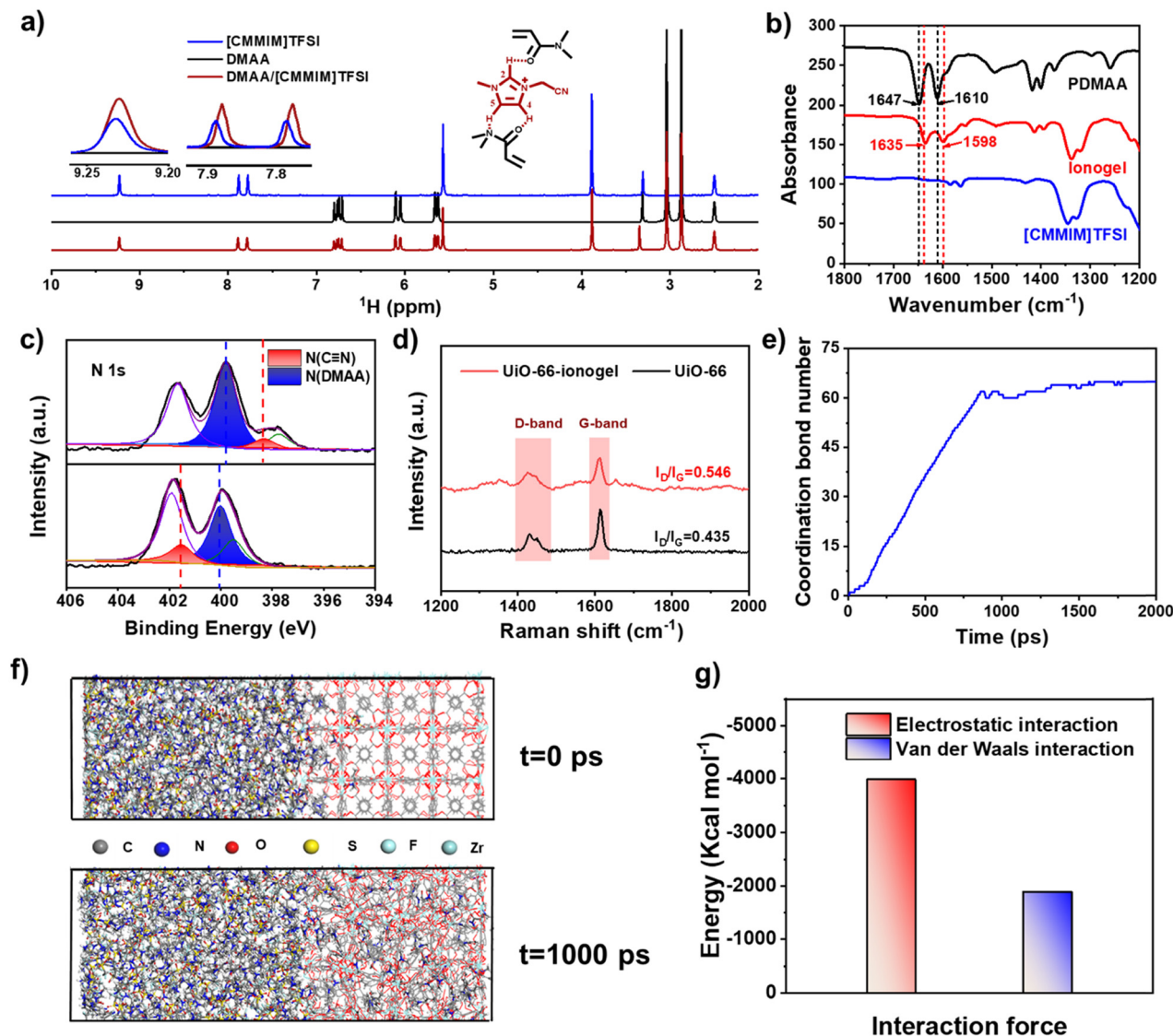
Fig. 1 Characterization of the reversible dynamic bonds in the UiO-66-ionogel. (a) 1 H NMR spectra of DMAA, [CMMIM]TFSI, and DMAA/[CMMIM]TFSI. The insets show hydrogen bonds between [CMMIM]TFSI and DMAA. (b) FT-IR spectra of PDMAA, [CMMIM]TFSI, and UiO-66-ionogel. (c) N 1s XPS results for the pure polymer and UiO-66/polymer. (d) Raman spectra of UiO-66 and UiO-66-ionogel. (e) Coordination bond number between UiO-66 and IL. (f) Snapshot of the MD system showing DMAA in UiO-66. (g) The energy of electrostatic and van der Waals interactions between DMAA and UiO-66 using MD simulations.
