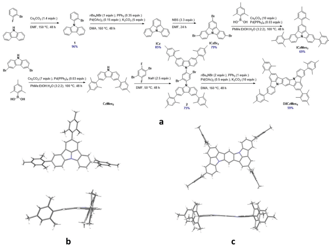
Fig. 4 Synthesis of (a) the emitters and crystal structures of (b) \text{ICzMes}_3 and (c) \text{DiICzMes}_4 .
