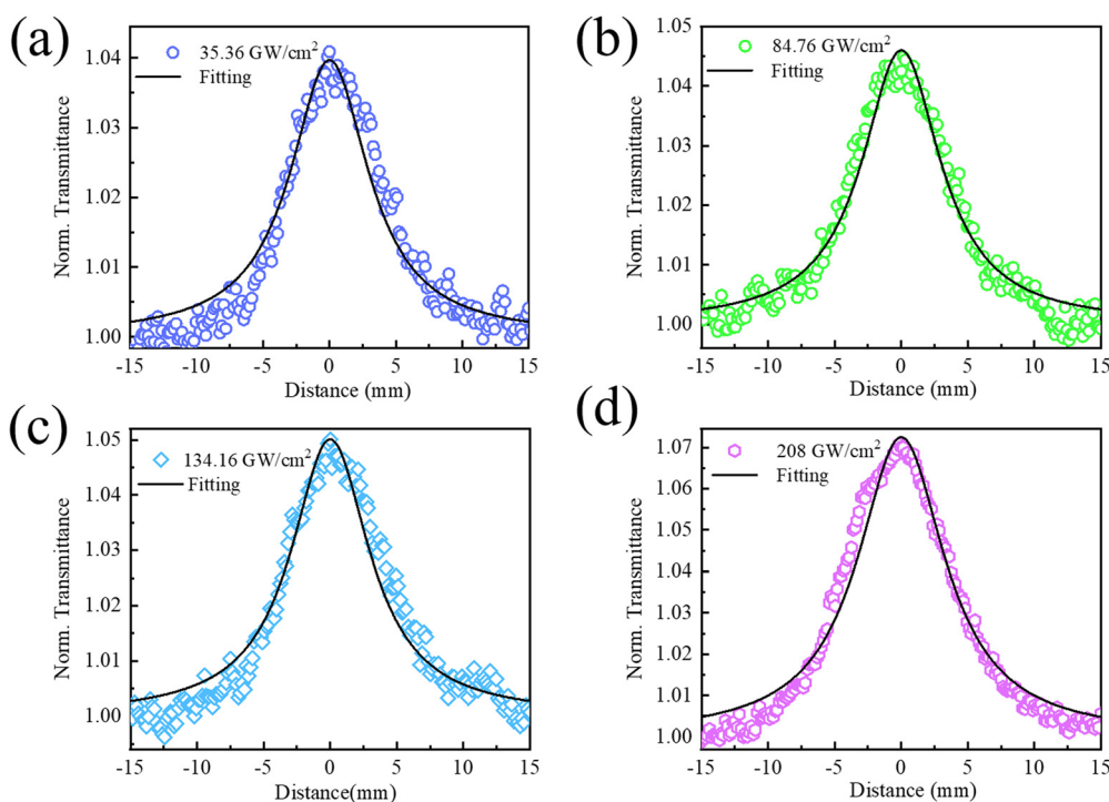
Fig. 4 Open aperture (OA) Z-scan curves obtained at an excitation wavelength of 800 nm for (a) 35.36, (b) 84.76, (c) 134.16 and (d) 208 \text{GW cm}^{-2} input intensities. The solid line in each figure represents the fitting of experimental data.
