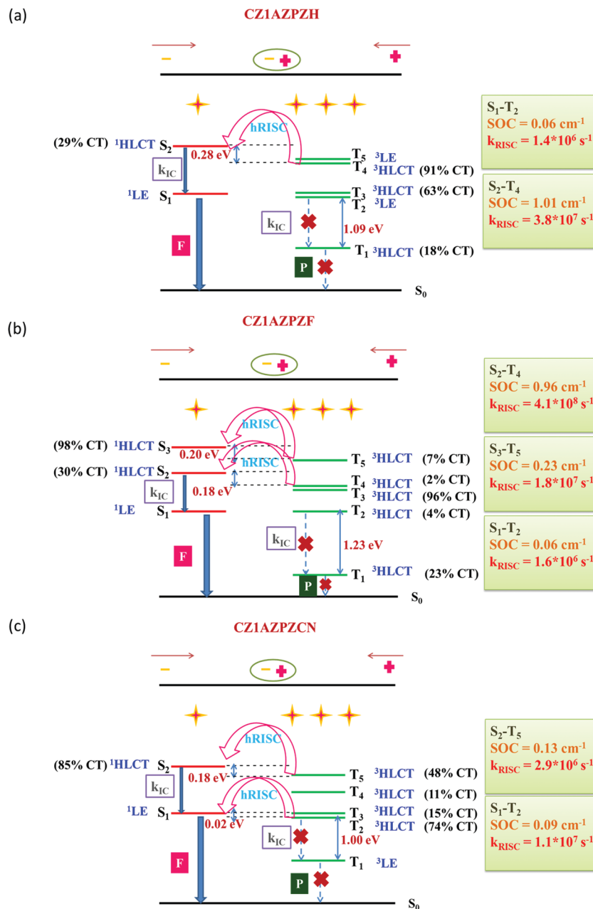
Fig. 5 Schematic depiction of a favourable hRISC process in (a) CZ1AZPZH, (b) CZ1AZPZF and (c) CZ1AZPZCN with the calculated energy levels, accompanying SOCs, and associated k_{\text{RISC}} .
