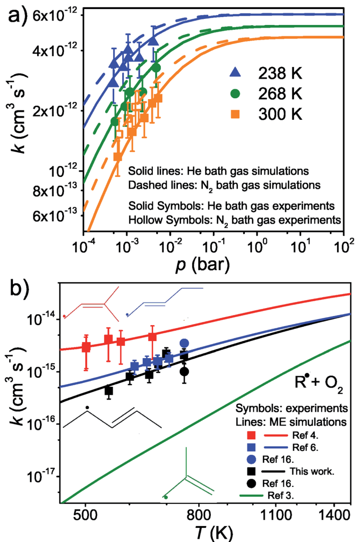
Fig. 4 This figure depicts the CH_3-CH=CH-CH_2-CH_3 + O_2 rate coefficient as a function of temperature and pressure. Below 300 K (a), the rate coefficient describes the CH_3-CH=CH-CH_2-CH_3 + O_2 \rightarrow CH_3-CH(OO^\bullet)-CH=CH-CH_3 recombination reaction. Above 500 K (b), the (phenomenological) rate coefficient describes the pressure independent CH_3-CH=CH-CH_2-CH_3 + O_2 \rightarrow bimolecular products reaction.
