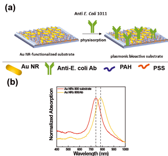
Fig. 5 Schematic of the procedure for bioactivating Au NR 800-functionalized substrates with the captured antibody able to recognize E. coli cells (a). Spectroscopic characterization of the bioactive plasmonic substrate after the incorporation of the Ab (yellow track) shows an optical red-shift of 40 nm with respect to the Au NR 800-functionalized substrate (b).
