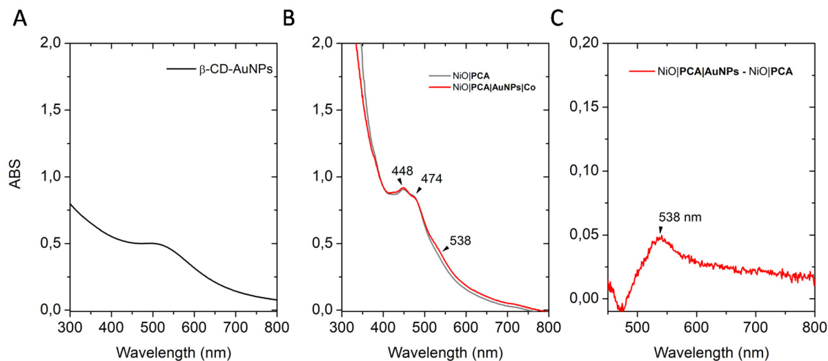
Fig. 2 Absorption UV-vis spectrum of (A) an aqueous solution of \beta\text{-CD-AuNPs} , (B) NiO|PCA (grey) and NiO|PCA| \beta\text{-CD-AuNPs} |Co (red) electrodes (NiO electrodes were used to set the background), and (C) Difference in absorption of NiO|PCA| \beta\text{-CD-AuNPs} and NiO|PCA electrodes.
