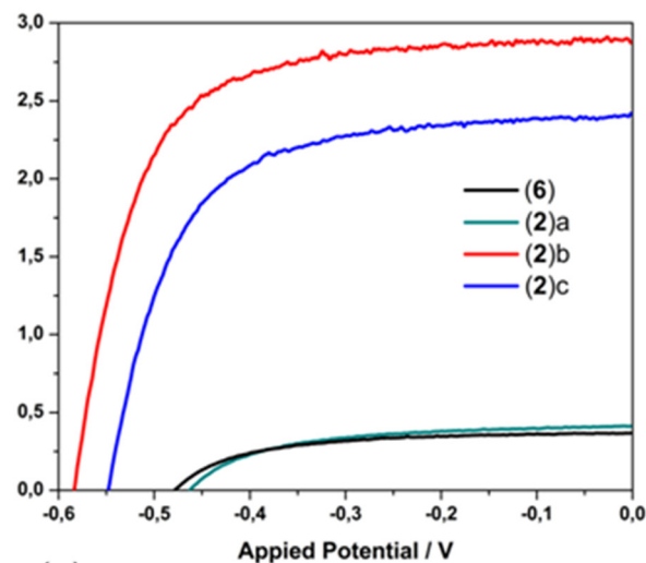
Fig. 13 J – V curves for the copper(I)-based dyes 1, [Cu(pqcame 2 )]PF 6 (A) (a); 2 and 6 (b). Lower case letters highlight the different architecture of the semiconductor material of the anode, dyed with 1 and 2, as reported in Table 2.
