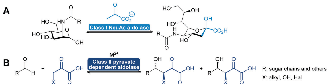
Scheme 8 (A) Already for more than 20 years pyruvate dependent aldolases are employed industrially to prepare N -acetylneuramic acid on a ton scale. (B) In recent years the scope of pyruvate dependent aldolases has been extended and they now activate also pyruvate derivatives and establish two stereocentres in one step. The stereoselectivity is, however, often determined by the product stability.
