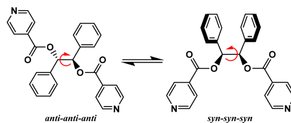
Scheme 1 Two possible conformations for 1,2-diphenylethane-1,2-diyl diisonicotinate (L).
