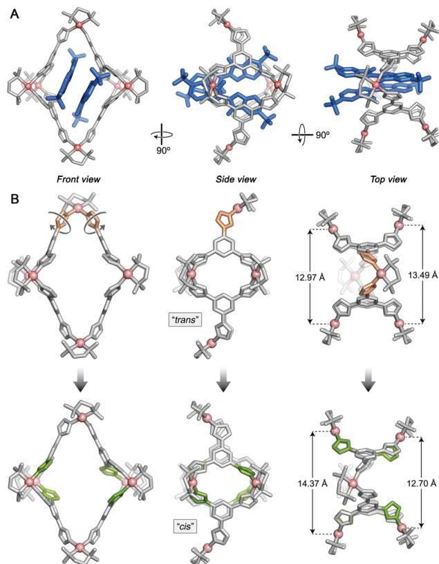
Fig. 3 (A) X-ray crystal structure of the 2_2\text{C}_1 inclusion complex viewed along three different directions. 1 , gray (with Pd in pink); 2 , blue. (B) Structural transformation of 1 accompanying encapsulation of 2 . Top panel: X-ray crystal structure of a typical G_2\text{C}_1 inclusion complex 29 (here, G = azobenzene, not shown for clarity). Bottom panel: X-ray crystal structure of 2_2\text{C}_1 ( 2 removed for clarity). The transformation is induced by a \sim 180^\circ rotation of the two axial imidazole groups shown in orange. The four imidazole groups highlighted in green are distorted from the plane of the central benzene ring significantly more than the other four equatorial imidazoles to more efficiently interact with the encapsulated 2 . Hydrogens, small ions, and water molecules were omitted for clarity.
