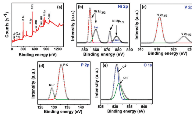
Fig. 4 (a) XP survey spectra and (b–e) XP spectra of the corresponding elements of NiVP/Pi after glucose oxidation.
