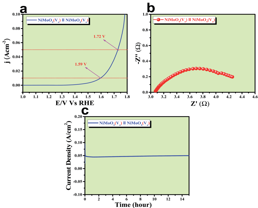
Fig. 10 (a) LSV curve of rod like \text{NiMoO}_4(\text{V}_o) as an anode and cathode in a two electrode system at a scan rate of 2 \text{ mV s}^{-1} , (b) impedance spectra obtained at 400 \text{ mV} overpotential, and (c) chronoamperometric outcomes for 15 hours.
