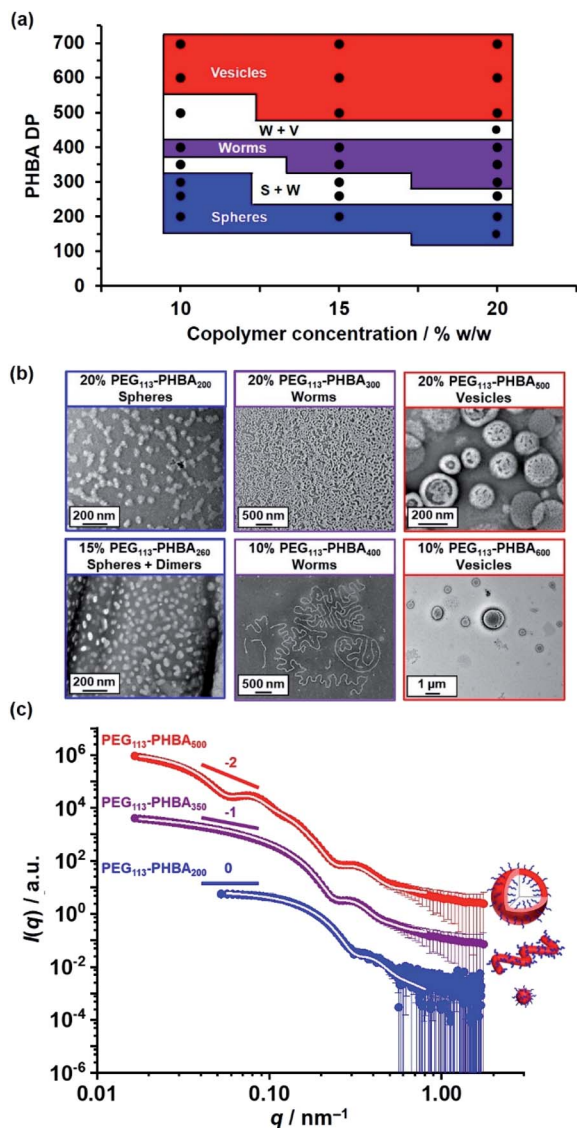
Fig. 4 (a) Pseudo-phase diagram constructed for a series of \text{PEG}_{113} - \text{PHBA}_x nano-objects synthesized via RAFT aqueous dispersion polymerization of HBA at 10%, 15% or 20% w/w solids based on a combination of TEM and DLS studies conducted at 20 °C (see Table S1† for the corresponding DLS data). S + W and W + V refer to sphere plus worm and worm plus vesicle mixed phases, respectively. (b) Representative TEM images recorded for a series of GA-crosslinked \text{PEG}_{113} - \text{PHBA}_x nano-objects after GA crosslinking at 20 °C using a [GA]/[HBA] molar ratio of 0.66. (c) Selected SAXS patterns (black, blue and red symbols) and corresponding data fits (solid white lines) obtained for 1.0% w/w aqueous copolymer dispersions of linear \text{PEG}_{113} - \text{PHBA}_{200} spheres, \text{PEG}_{113} - \text{PHBA}_{350} worms and \text{PEG}_{113} - \text{PHBA}_{600} vesicles at 20 °C and pH 7. See Table S1† for a summary of the nano-object dimensions calculated using the appropriate scattering models. 80,81
