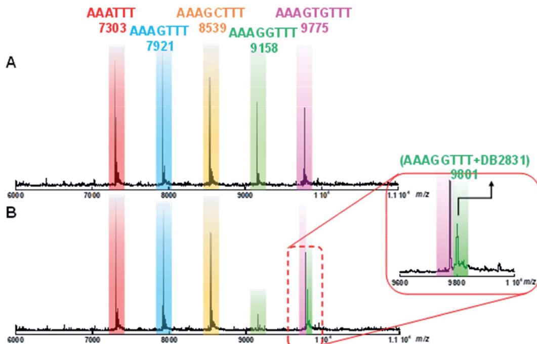
Fig. 5 ESI-MS negative mode spectra of the competition binding of sequences AAATTT; AAAGTTT; AAAGCTTT; AAAGGTTT; AAAGTGTTC: (10 \mu M each); with 40 \mu M DB2831 in buffer (50 mM ammonium acetate with 10% methanol (v/v), pH 6.8). (A) The ESI-MS spectra of free DNA mixture. (B) The ESI-MS spectra of DNA mixture with compounds. The ESI-MS results shown here are deconvoluted spectra and molecular weights are shown with each peak. The inset in red box is the expansion of (B) between 9600 and 10 000 m/z .
