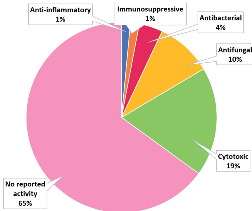
Fig. 12 Biological activity spectrum of cerebroside isolations from the studied marine organisms.
