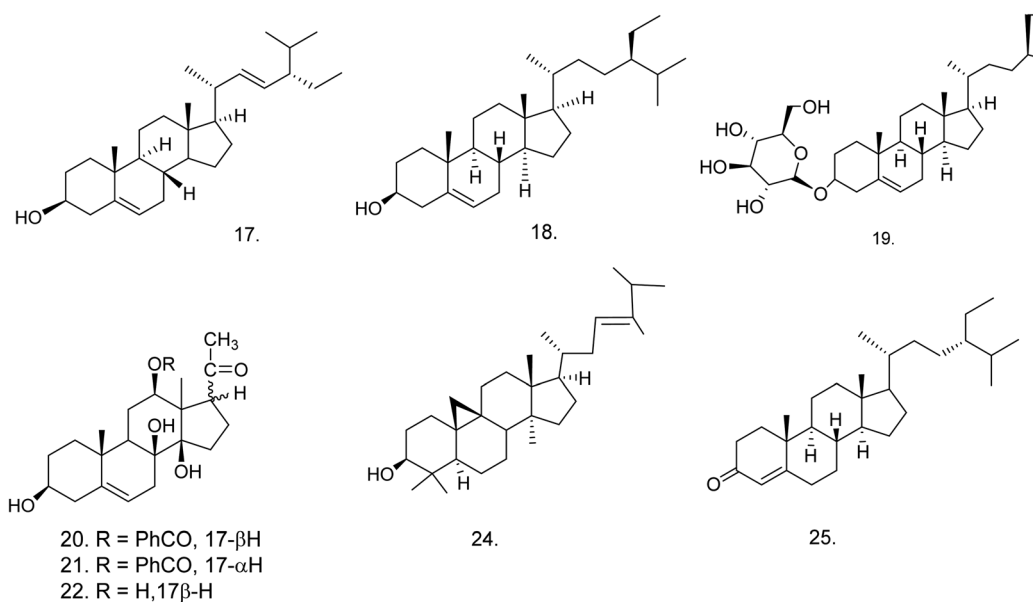
Fig. 2 Chemical structures of steroids.
