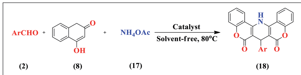
Scheme 15 Catalytic synthesis of coumarin containing 1,4-DHPs.
