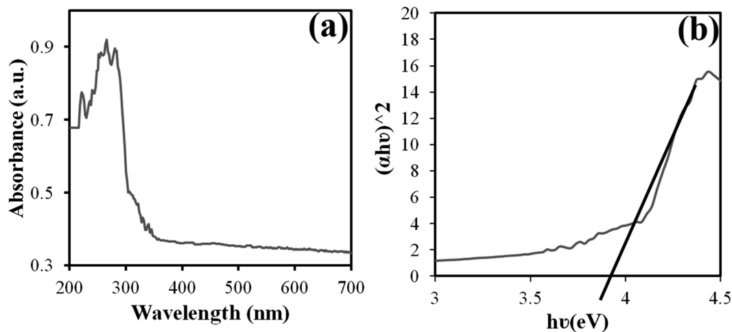
Fig. 5 Graphs of (a) DRS and (b) (\alpha hv)^2 versus hv for the band gap estimate obtained from sample no. 3.
