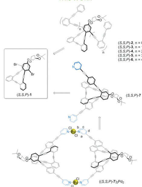
Fig. 1 Top: Previous studies with foldamers and helicene-type systems with more than two loops. Bottom: New helical systems developed in this work: chemical structure of stapled nucleus (S,S,P)-1, helical systems (S,S,P)-2–(S,S,P)-6, ligand (S,S,P)-7 and metallosupramolecular complex ((S,S,P)-7) 2 Pd 2 .
