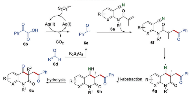
Scheme 6 The construction of the carbonyl-containing quinoline-2,4-diones.
