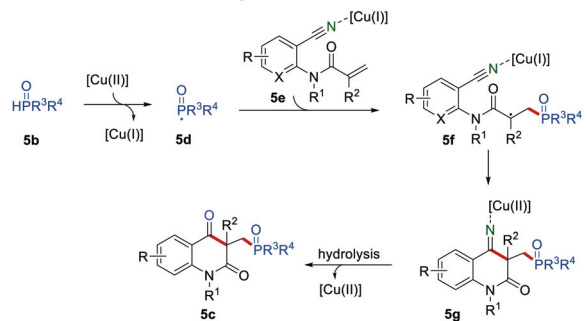
Scheme 5 The preparation of the phosphorylated quinoline-2,4-diones.
