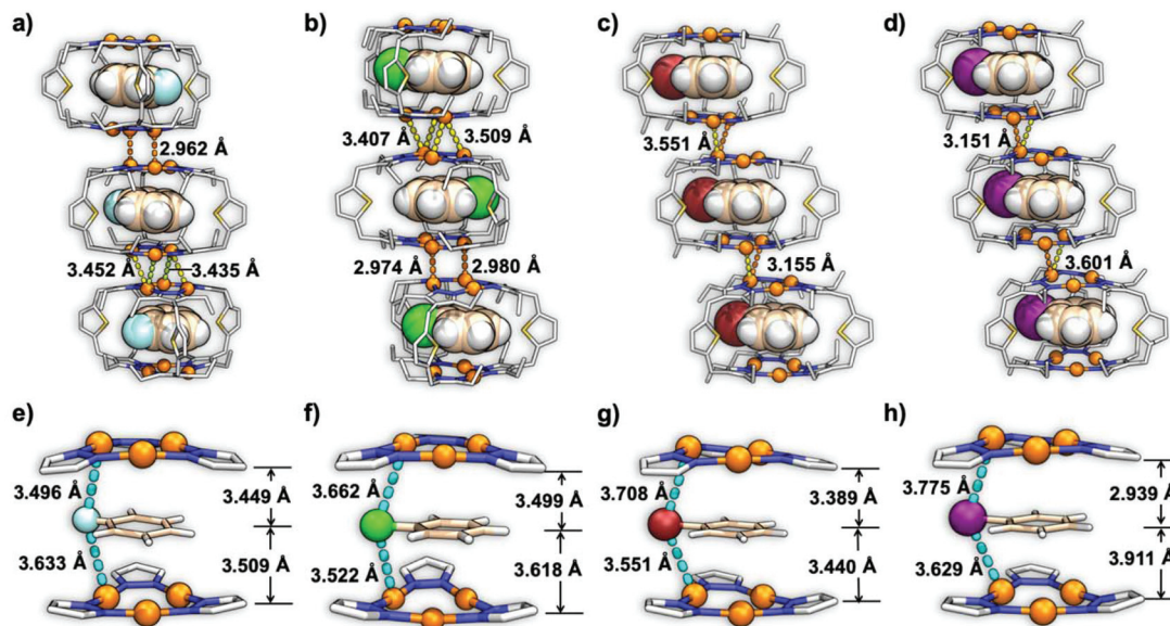
Fig. 1 Crystal structures of (a) 1D Ph-F, (b) 1D Ph-Cl, (c) 1D Ph-Br, and (d) 1D Ph-I, showing the Cu 3 L 6 cage units in one packed column with intermolecular Cu...Cu distances of 2.962, 3.452 and 3.435 Å in 1D Ph-F, 3.407, 3.509, 2.974 and 2.980 Å in 1D Ph-Cl, 3.551 and 3.155 Å in 1D Ph-Br, and 3.151 and 3.601 Å in 1D Ph-I, respectively (Cu(I) ions, cage hosts 1, and halobenzene guests are shown as the ball, line and space-filling model, respectively; hydrogen atoms in cage hosts 1 are omitted for clarity; C, N, S, and Cu atoms in the cage are shown in gray, blue, yellow, and orange colours, respectively; C, H, F, Cl, Br and I atoms in the guests are shown in wheat, white, light cyan, green, brown and purple colours, respectively); CTC-guest-CTC structures of (e) 1D Ph-F, (f) 1D Ph-Cl, (g) 1D Ph-Br, and (h) 1D Ph-I, showing intermolecular Cu...X distances of 3.496 and 3.633 Å in 1D Ph-F, 3.662 and 3.522 Å in 1D Ph-Cl, 3.708 and 3.551 Å in 1D Ph-Br, and 3.775 and 3.629 Å in 1D Ph-I, respectively (Cu(I) ions, halogen atoms, CTC units, and guests are shown as the ball and line model, respectively).
