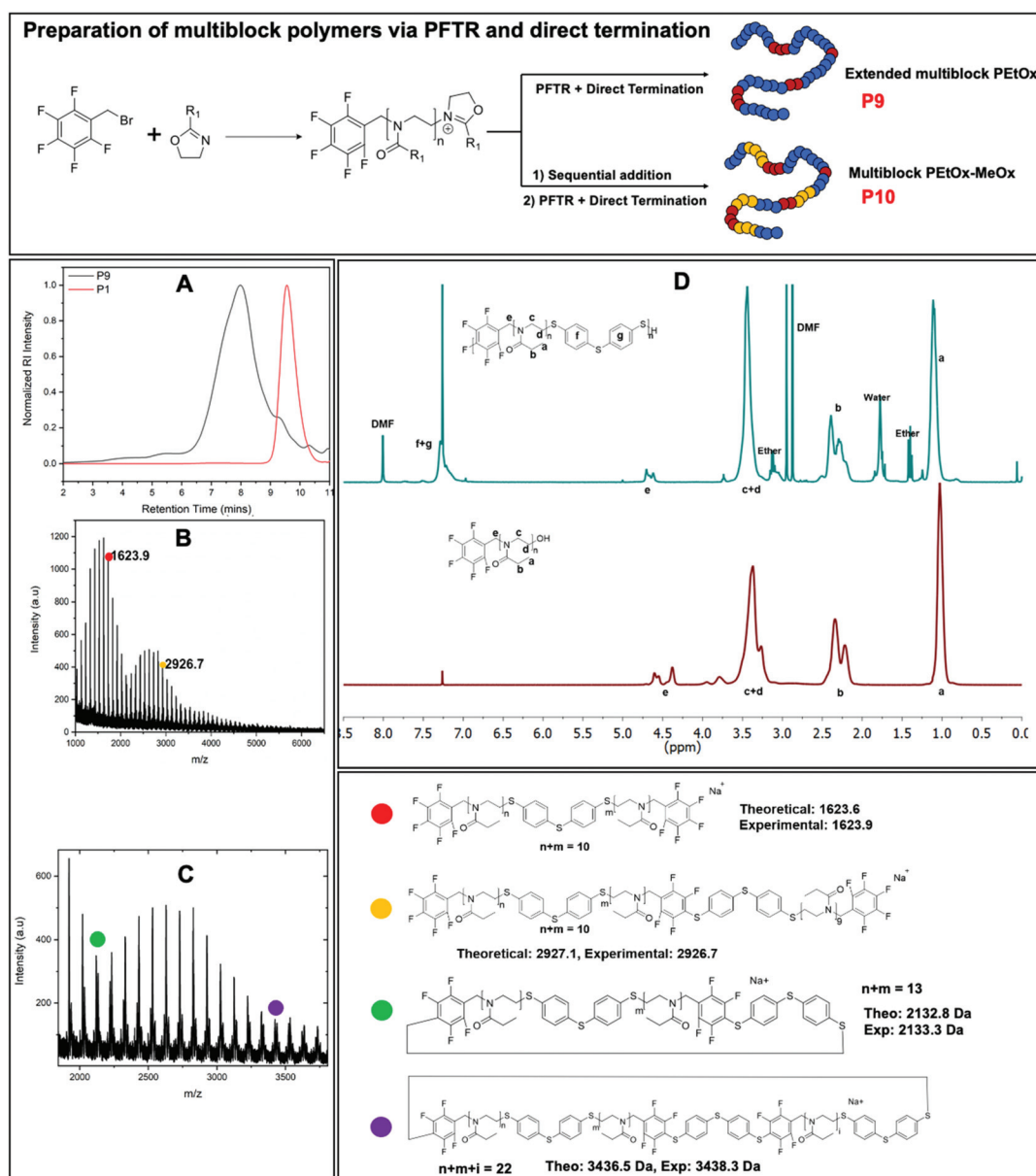
Fig. 4 Preparation of multiblock PETox and characterization of extended multiblock polymer P9 with SEC (A), MALDI-ToF MS (B), zoom in to the high molar mass region in the MALDI-ToF MS (C), and ^1\text{H} NMR (D) showing the growth of multiblock polymer and possible cyclic structure formation (green and purple).
