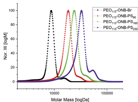
Fig. 2 GPC traces of PEO 113 -ONB-Br macroinitiator, PEO 113 -ONB-PS 90 , PEO 113 -ONB-PS 165 , and PEO 113 -ONB-PS 230 .
