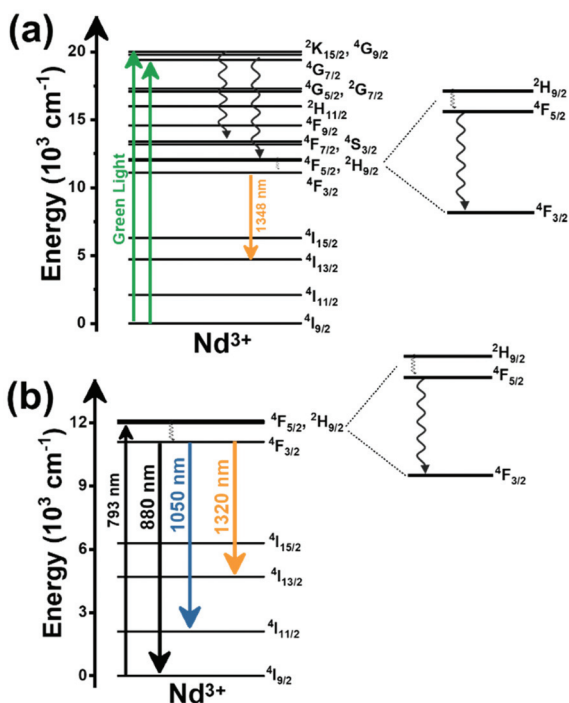
Fig. 30 Mechanisms of generation of the: (a) 1348 nm emission band in \text{Nd}^{3+}:\text{YAP} nanoparticles under green light excitation, and (b) 1050 nm and 1320 nm emission bands in \text{Nd}^{3+}:\text{LiLuF}_4@/\text{LiLuF}_4 nanoparticles under 793 nm excitation.
