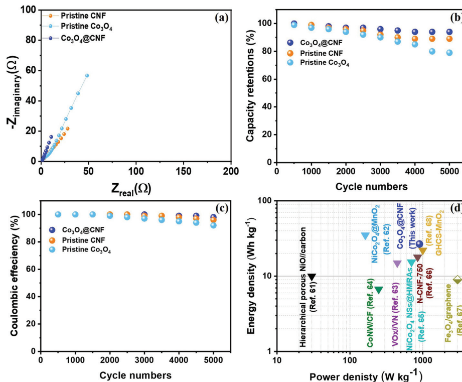
Fig. 7 Electrochemical performance of the SSC devices for the pristine \text{Co}_3\text{O}_4 nanoparticles, pristine CNF and 1D \text{Co}_3\text{O}_4@CNF hybrid electrodes: (a) EIS plot, (b and c) capacity of retentions and coulombic efficiency of electrodes at 15 \text{ A g}^{-1} of current density over 5000 cycles and (d) Ragone plot.
