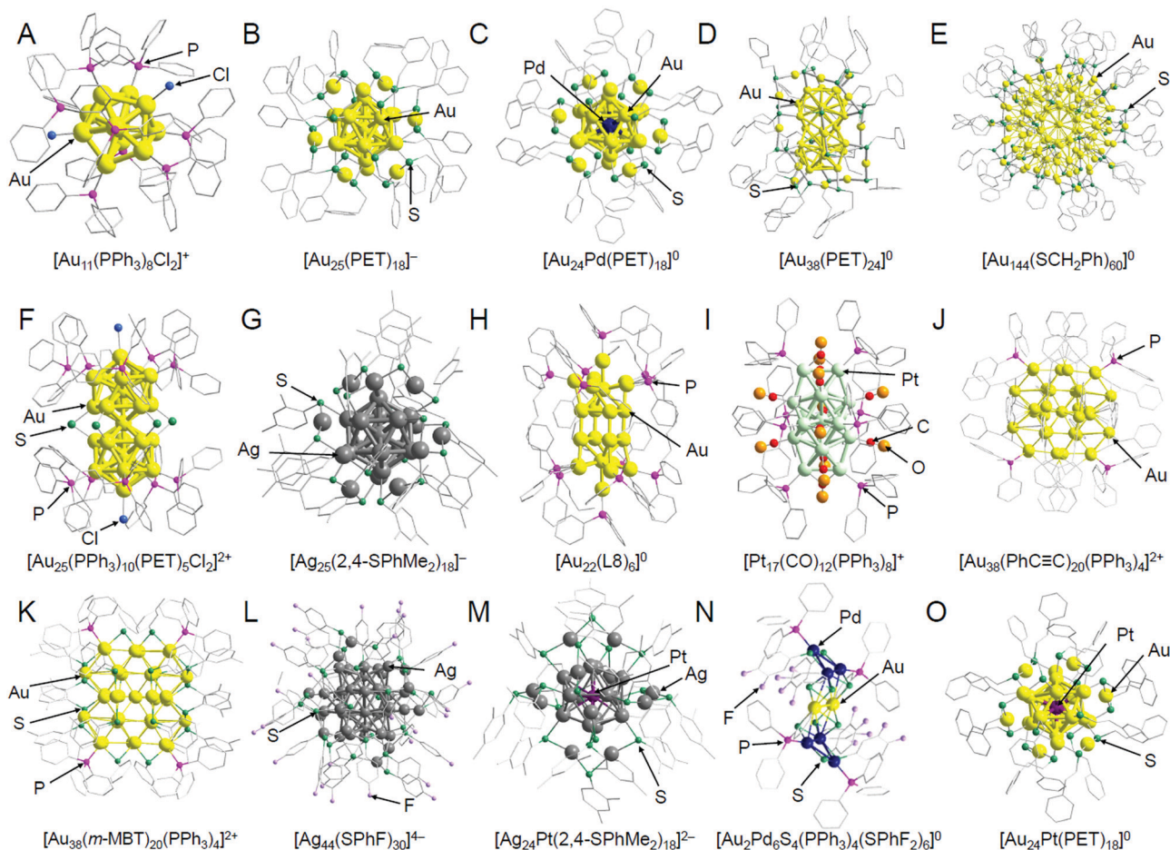
Fig. 2 Geometrical structures of atompically precise, ligand-protected metal NCs: (A) [\text{Au}_{11}(\text{PPh}_3)_8\text{Cl}_2]^+ , 171 (B) [\text{Au}_{25}(\text{PET})_{18}]^- , 42 (C) [\text{Au}_{24}\text{Pd}(\text{PET})_{18}]^0 , 172 (D) [\text{Au}_{38}(\text{PET})_{24}]^0 , 173 (E) [\text{Au}_{144}(\text{SCH}_2\text{Ph})_{60}]^0 , 174 (F) [\text{Au}_{25}(\text{PPh}_3)_{10}(\text{PET})_5\text{Cl}_2]^{2+} , 175 (G) [\text{Ag}_{25}(2,4\text{-SPhMe}_2)_{18}]^- , 43 (H) [\text{Au}_{22}(\text{L}8)_6]^0 , 176 (I) [\text{Pt}_{17}(\text{CO})_{12}(\text{PPh}_3)_8]^+ , 177 (J) [\text{Au}_{38}(\text{PhC}\equiv\text{C})_{20}(\text{PPh}_3)_4]^{2+} , 178 (K) [\text{Au}_{38}(m\text{-MBT})_{20}(\text{PPh}_3)_4]^{2+} , 178 (L) [\text{Ag}_{44}(\text{SPhF})_{30}]^{4+} , 44 (M) [\text{Ag}_{24}\text{Pt}(2,4\text{-SPhMe}_2)_{18}]^{2-} , 179 (N) [\text{Au}_2\text{Pd}_6\text{S}_4(\text{PPh}_3)_4(\text{SPhF}_2)_6]^0 , 180 and (O) [\text{Au}_{24}\text{Pt}(\text{PET})_{18}]^0 . 26 The gray points indicate carbon atoms, and hydrogen atoms are not shown. \text{Au}_{25}(\text{SR})_{18} (SR = SC12 or SG) discussed in Sections 2.1.1, 2.1.2, and 2.4 is considered to have a similar geometrical structure as [\text{Au}_{25}(\text{PET})_{18}]^- (B). \text{Au}_{24}\text{Pd}(\text{SC}12)_{18} discussed in Section 2.1.1 is considered to have a similar geometrical structure as [\text{Au}_{24}\text{Pd}(\text{PET})_{18}]^0 (C). \text{Au}_{38}(\text{SC}12)_{24} discussed in Section 2.1.4 is considered to have a similar geometrical structure as [\text{Au}_{38}(\text{PET})_{24}]^0 (D). \text{Au}_{144}(\text{PET})_{60} discussed in Sections 2.1.1–2.1.4 is considered to have a similar geometrical structure as [\text{Au}_{144}(\text{SCH}_2\text{Ph})_{60}]^0 (E). These graphics were reproduced with permission from ref. 26, 42–44 and 171–180. Copyright 2016 Royal Society of Chemistry, 2008 American Chemical Society, 2015 American Chemical Society, 2013 Springer-Nature, 2014 American Chemical Society, 2016 American Chemical Society, 2010 American Chemical Society, 2018 AAAS, 2007 American Chemical Society, 2014 American Chemical Society, 2017 American Chemical Society, 2017 AAAS, 2017 American Chemical Society, 2018 Royal Society of Chemistry, respectively.
