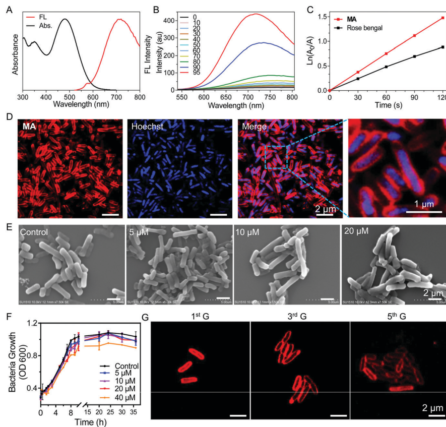
Fig. 1 (A) Normalized absorption and fluorescence (FL) spectra of MA in DMSO and water (v/v = 1/99) solution. (B) FL spectra of MA (10 μM) in DMSO/toluene mixtures with different volume fractions (v/v); \lambda_{\text{exc}} : 488 nm. (C) Decomposition rates of ABDA induced by ROS generated from MA (10 μM) under white light irradiation (30 mW cm -2 ) in DMSO/water (v/v = 1/99) solution. [ABDA] = 5 \times 10^{-5} M, time interval for recording the UV-vis spectra: 30 s. (D) Confocal microscopy images of metabolically labeled Salmonella (20 μM MA for 30 min). (E) Field emission scanning electron microscopy images of Salmonella labelled with various concentrations of MA . The control group is the untreated Salmonella . (F) The bacterial growth of MA labelled Salmonella in fresh LB solution. (G) Confocal microscopy images of MA labelled Salmonella at different cell generation cycles in fresh LB solution.
