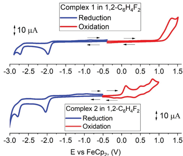
Fig. 2 Cyclic voltammograms for 1 (top) and 2 (bottom), recorded in 1,2-difluorobenzene solution (1.4 mM) with [n\text{-Bu}_4\text{N}]\text{PF}_6 as supporting electrolyte (0.13 M) using a glassy carbon electrode, scan rate 0.1 \text{Vs}^{-1} .
